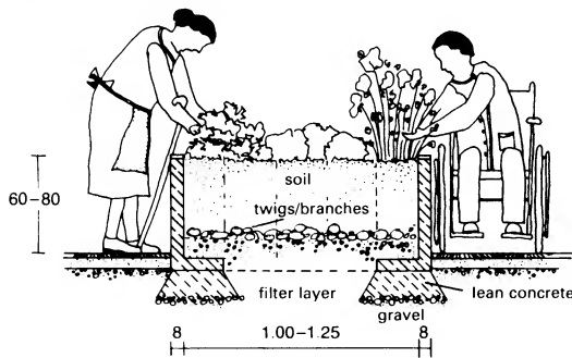
8 Raised bed made from prefabricated concrete units
